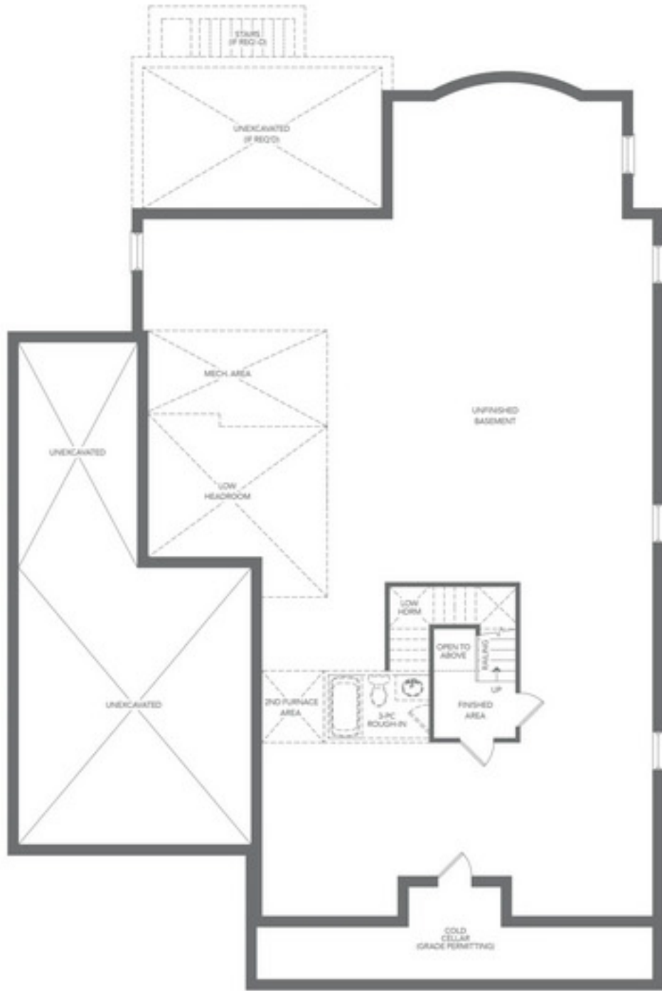
ELEVATION A | BASEMENT
